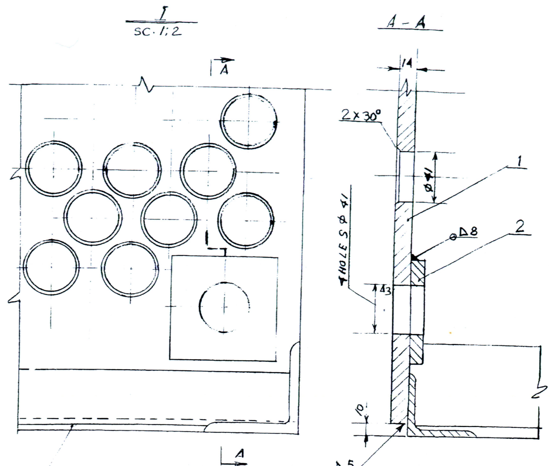
FRAME POS. NO. 8 DRG. NO. 085.001.00.033 SHOWN CONVENTIONALLY IN ASSLY. WITH BED PLATE (LOWER)
