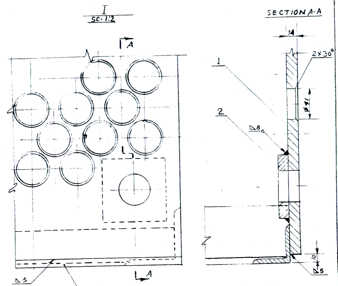
FRAME POS. NO. - 6. DRG. NO. 085.001.00.033 SHOWN CONVENTIONALLY IN ASSLY. WITH BED PLATE (TOP)
