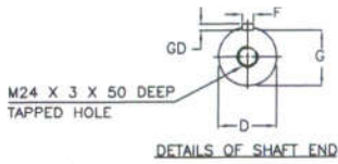
DETAILS OF SHAFT END
